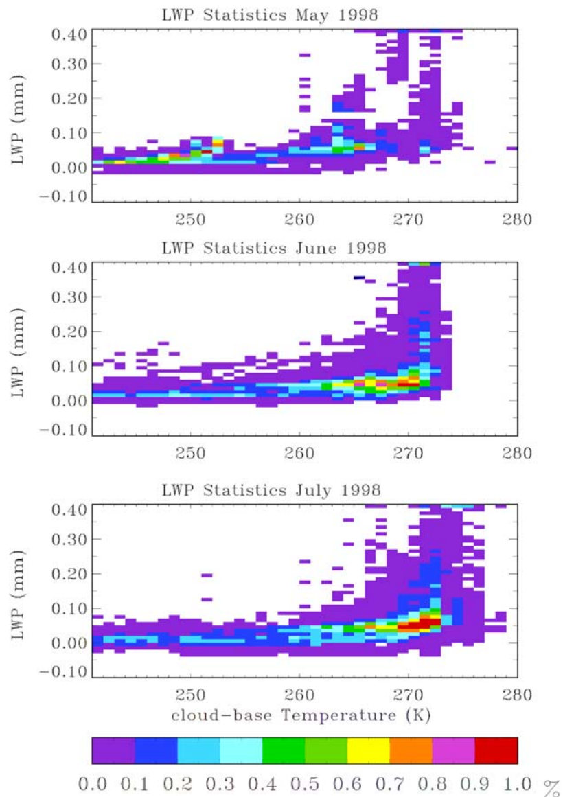
Figure 7. Statistics on LWP and cloud base temperature for May, June, and July 1998.
