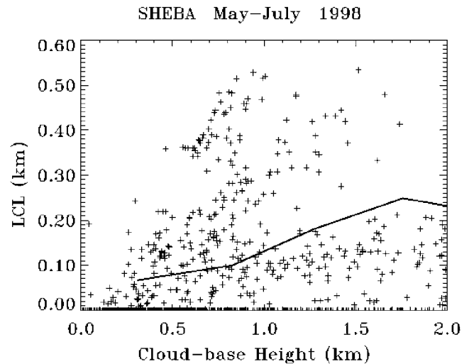
Figure 11. Scatterplot of LCL and observed cloud base height. The solid curve is for the averages of cloud base height binned in every half-kilometer.
