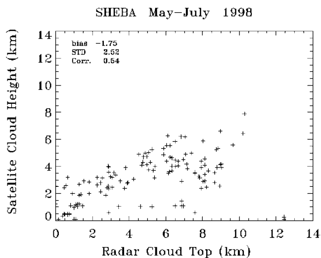
Figure 1. Scatterplot of MMCR estimated cloud top height with satellite estimated cloud top height.
