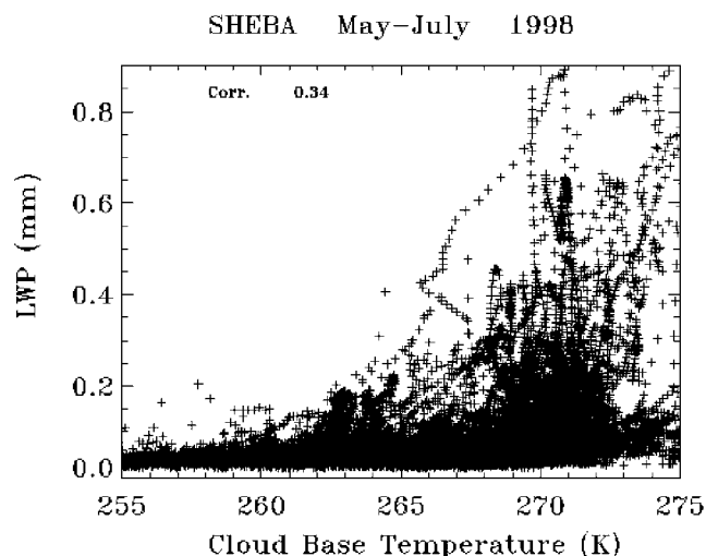
Figure 2. The relationship between cloud liquid water path (LWP) and cloud base temperature.
