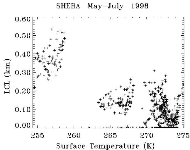
Figure 9. Temperature dependence of cloud lifting condensation level (LCL). The LCL values were theoretically estimated from surface meteorological measurements of temperature and humidity and atmospheric profile.
