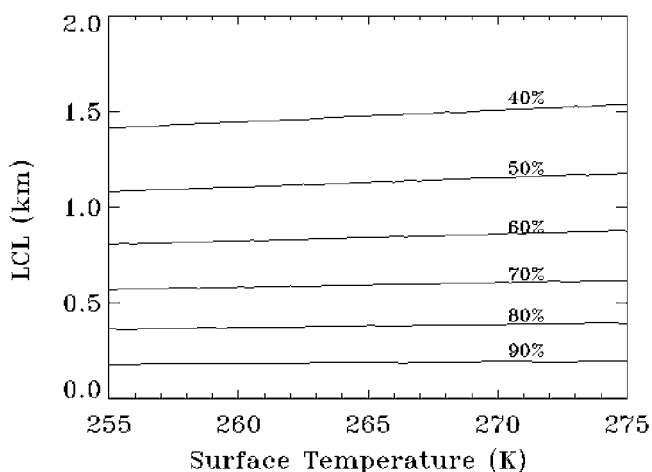
Figure 10. Theoretically estimated LCL for different relative humidities in the surface air temperature range from 255 K to 275 K.
