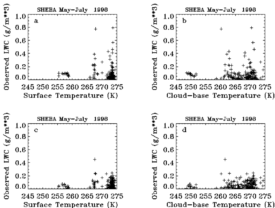
Figure 4. Scatterplot of LWC with surface temperature (Figure 4a) and cloud base temperature (Figure 4b). Figures 4c and 4d are the same as Figures 4a and 4b, respectively, except the cloud thickness data from MMCR are used in LWC calculations.
