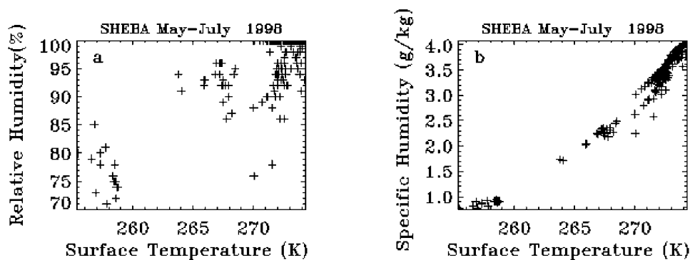
Figure 8. Surface air temperature dependence of relative humidity (Figure 8a) and specific humidity (Figure 8b).
