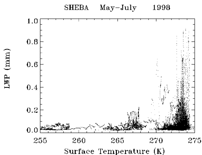
Figure 5. Same as Figure 2, except for surface air temperature.
