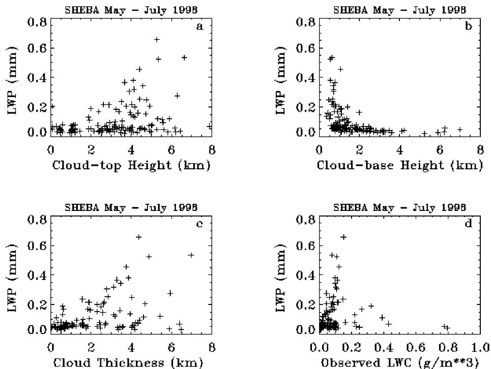
Figure 3. LWP dependence on cloud top height (Figure 3a), cloud base height (Figure 3b), cloud thickness (Figure 3c) and cloud liquid water content LWC (Figure 3d).
