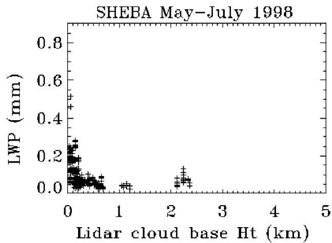
Figure 6. The relationship between LWP and cloud base height observed by DABUL.
